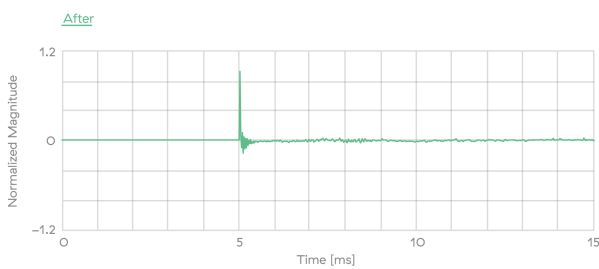
Impulse response before and after Dirac Live Correction
