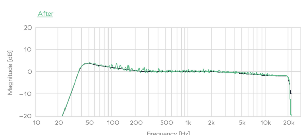
Frequency response before and after Dirac Live Correction
